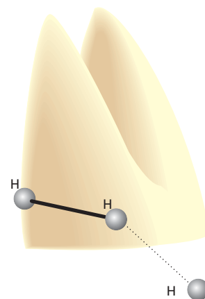
Fig. 24.19 An indication of the anisotropy of the potential energy changes as H_2 approaches H with different angles of attack. The collinear attack has the lowest potential barrier to reaction. The surface indicates the potential energy profile along the reaction coordinate for each configuration.
