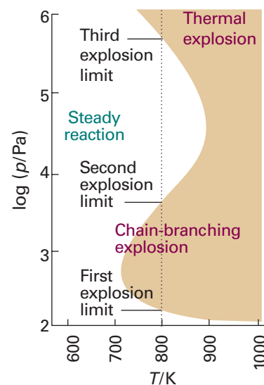
Fig. 23.3 The explosion limits of the \text{H}_2 + \text{O}_2 reaction. In the explosive regions the reaction proceeds explosively when heated homogeneously.
