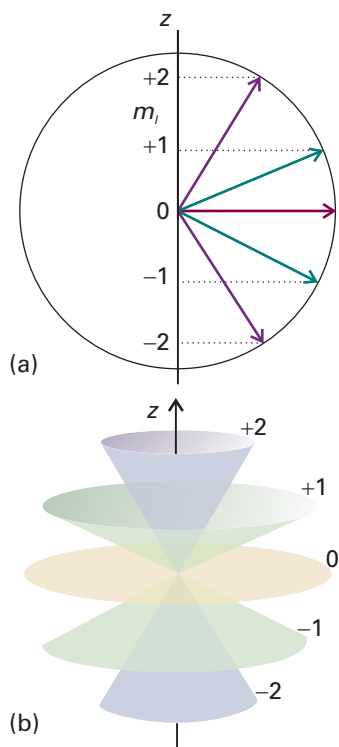
Fig. 9.40 (a) A summary of Fig. 9.38. However, because the azimuthal angle of the vector around the z-axis is indeterminate, a better representation is as in (b), where each vector lies at an unspecified azimuthal angle on its cone.
