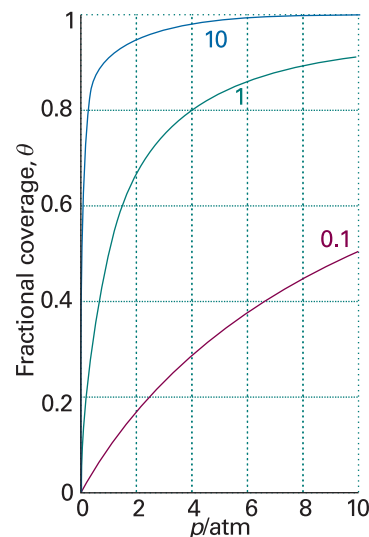
Fig. 25.16 The Langmuir isotherm for dissociative adsorption, \text{X}_2(\text{g}) \rightarrow 2 \text{X}(\text{surface}) , for different values of K .
