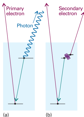
Fig. 25.10 When an electron is expelled from a solid (a) an electron of higher energy may fall into the vacated orbital and emit an X-ray photon to produce X-ray fluorescence. Alternatively, (b) the electron falling into the orbital may give up its energy to another electron, which is ejected in the Auger effect.
